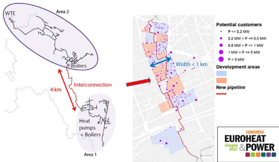
Figure 26 Plan of the separated district heating networks, source: www.4dh.eu
